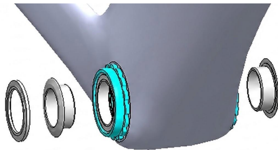
Drive Side 3mm+29mm dust cover
